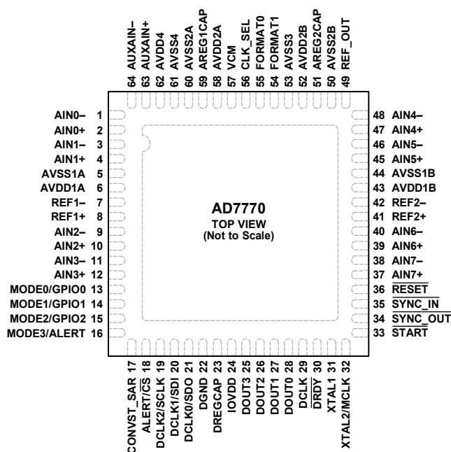
Figure 7. Pin Configuration
