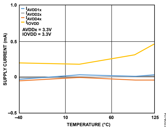
Figure 97. Shutdown Current
