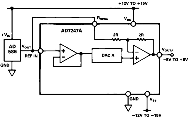
Figure 9. Bipolar Configuration
