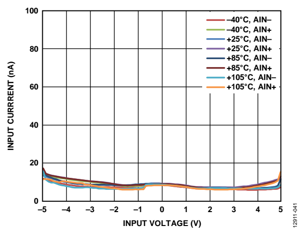
Figure 40. Analog Input Current vs. Input Voltage ( V_{CM} = 2.5 V )
