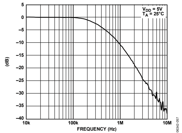
Figure 51. Multiplying Bandwidth
