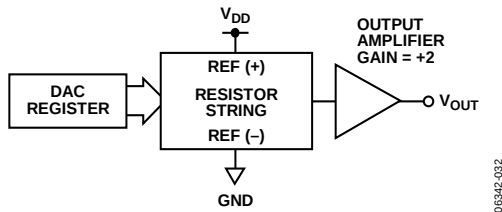
Figure 52. DAC Architecture
