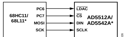
Figure 35. AD5512A/AD5542A to 68HC11/68L11 Interface
