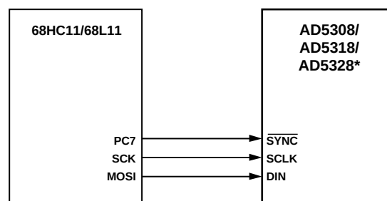
Figure 37. 68HC11/68L11-to-AD5308/AD5318/AD5328 Interface
