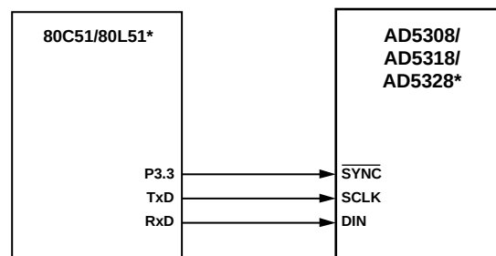
Figure 38. 80C51/80L51-to-AD5308/AD5318/AD5328 Interface
