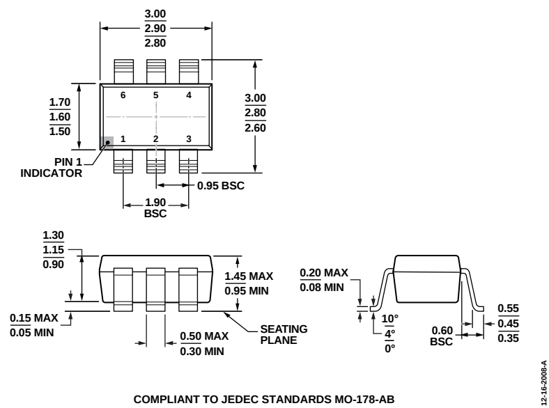
Figure 33. 6-Lead Small Outline Transistor Package (SOT-23) (RJ-6) Dimensions shown in millimeters
