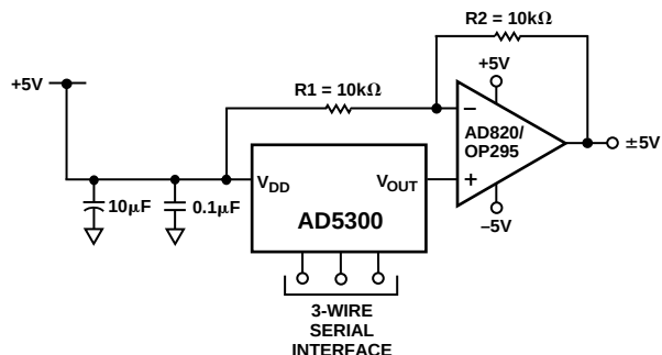
Figure 30. Bipolar Operation with the AD5300
