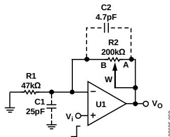
Figure 59. Typical Noninverting Gain Amplifier
