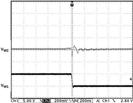
Figure 23. Digital Crosstalk
