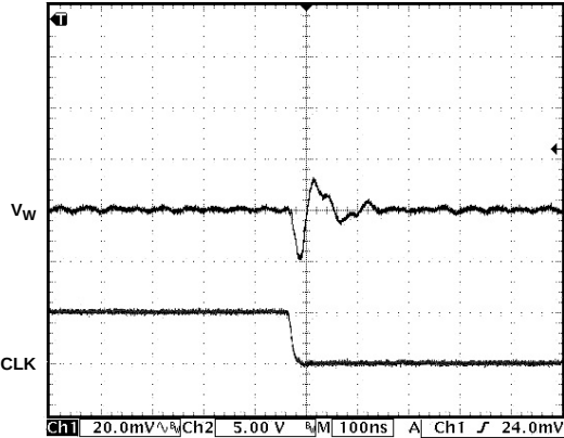
Figure 22. Digital Feedthrough
