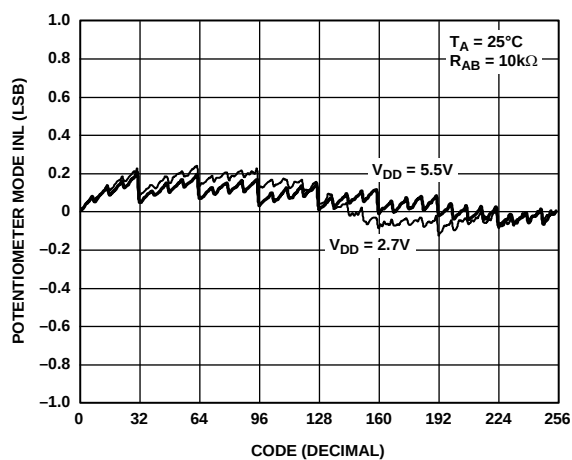
Figure 7. INL vs. Code vs. Supply Voltages
