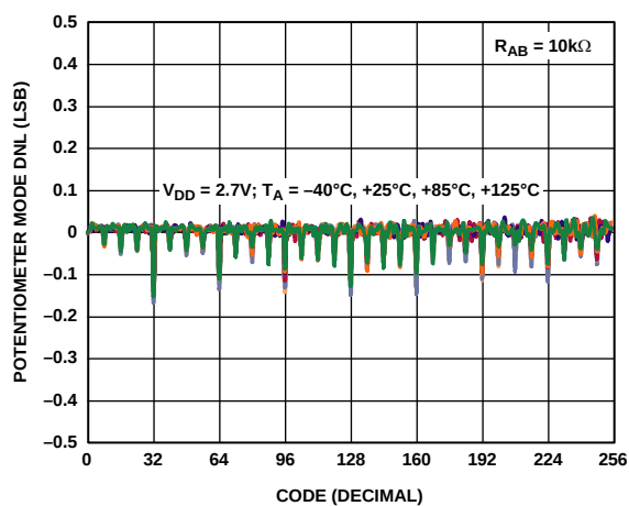
Figure 6. DNL vs. Code vs. Temperature
