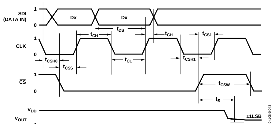
Figure 43. SPI Interface Detailed Timing Diagram ( V_A = 5\text{ V} , V_B = 0\text{ V} , V_W = V_{OUT} )
