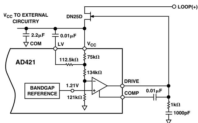
Figure 3. AD421 Voltage Regulator Circuit to Provide V_{CC} = 3.3\text{ V}
