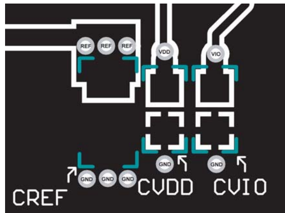
Figure 66. Example Layout of the AD4000 (Bottom Layer)
