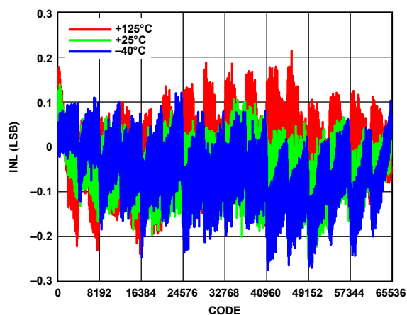
Figure 7. INL vs. Code for Various Temperatures, V_{REF} = 2.5\text{ V}
