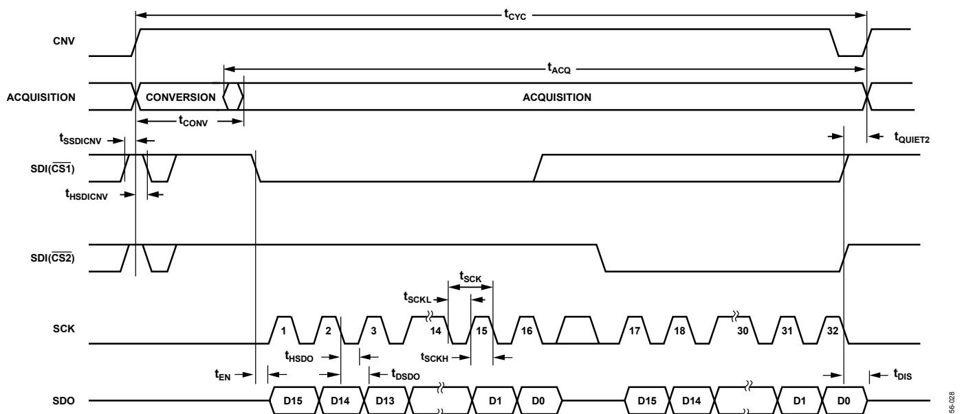
Figure 60. \overline{\text{CS}} Mode, 4-Wire Without Busy Indicator Serial Interface Timing Diagram (Status Bits Not Shown)
