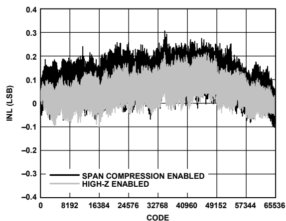
Figure 8. INL vs. Code, High-Z and Span Compression Modes, V_{REF} = 5\text{ V}
