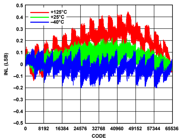
Figure 6. INL vs. Code for Various Temperatures, V_{REF} = 5\text{ V}
