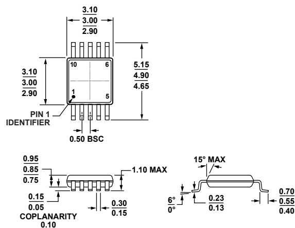
Figure 67. 10-Lead Mini Small Outline Package [MSOP] (RM-10)
