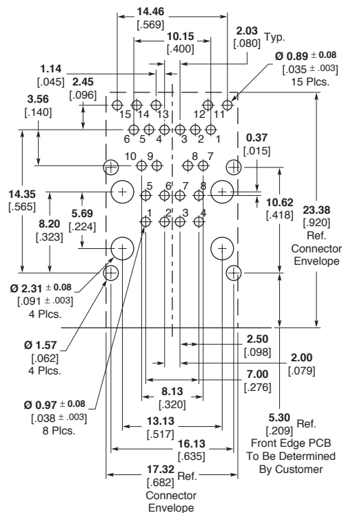
PCB Footprint
