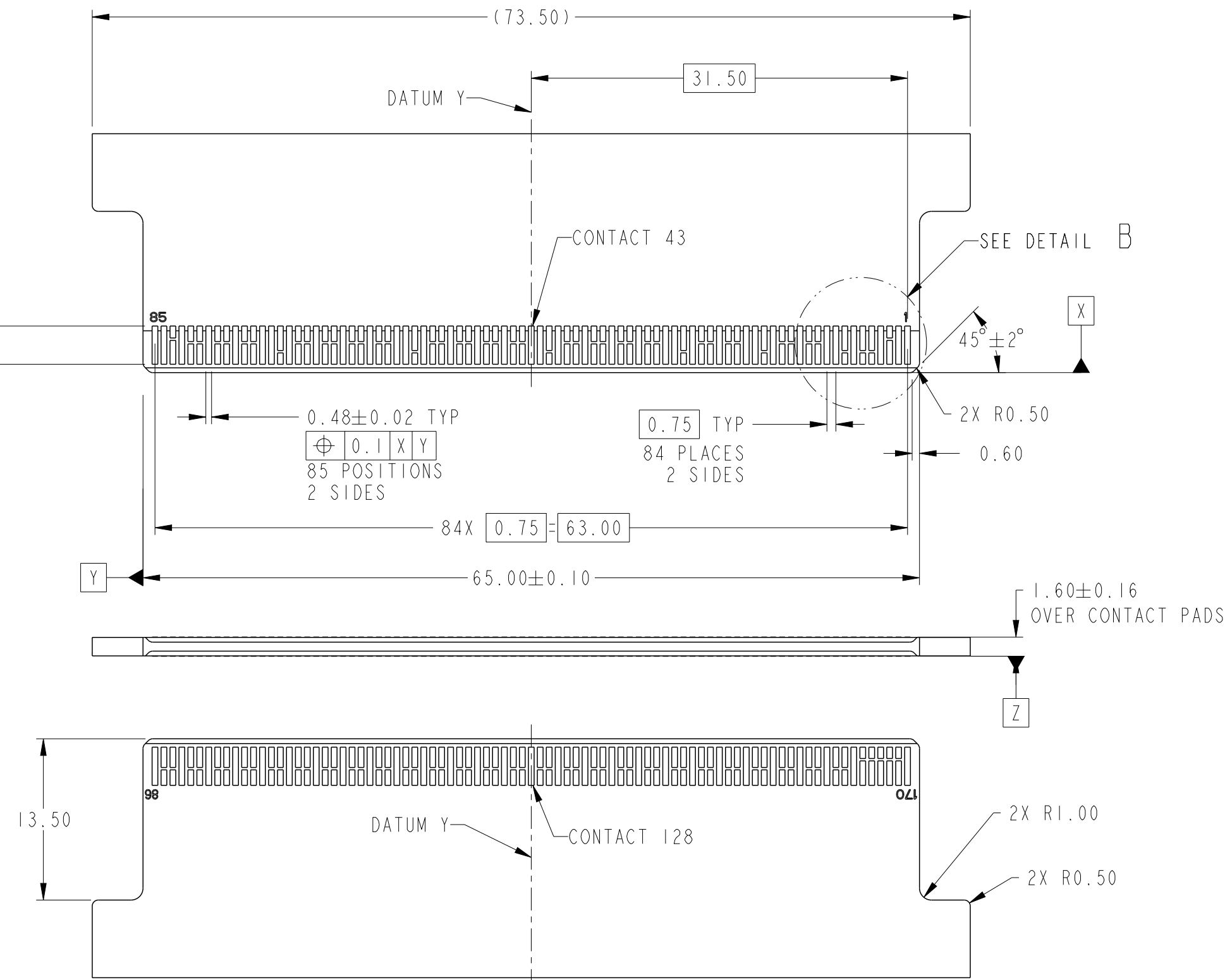
SCALE 5:2 RECOMMENDED MODULE CARD-EDGE INTERFACE DIMENSIONS
