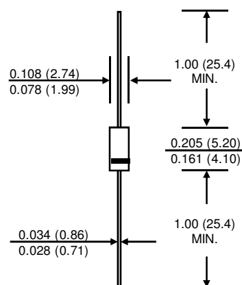
DO-41
