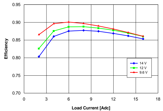
Fig. 1.5V.2: Efficiency vs. load current and input voltage for V_{out} = 1.5\text{ V} converter mounted vertically with air flowing at a rate of 200\text{ LFM} ( 1\text{ m/s} ) and T_a = 25\text{ }^{\circ}\text{C} .
