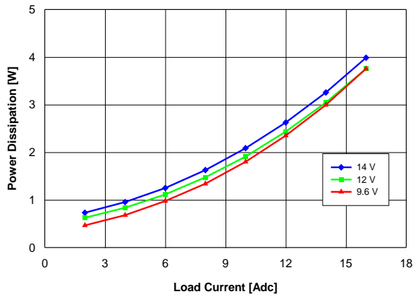
Fig. 1.5V.3: Power loss vs. load current and input voltage for V_{out} = 1.5\text{ V} converter mounted vertically with air flowing at a rate of 200\text{ LFM} ( 1\text{ m/s} ) and T_a = 25\text{ }^{\circ}\text{C} .
