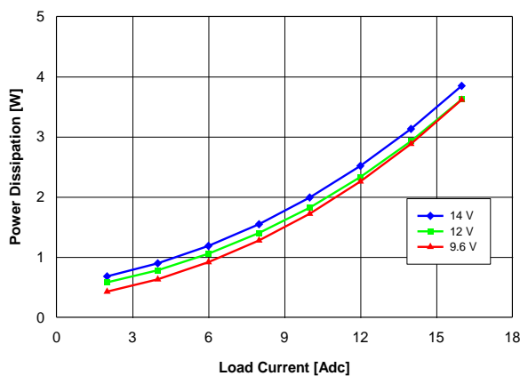
Fig. 1.0V.3: Power loss vs. load current and input voltage for V_{out} = 1.0 V converter mounted vertically with air flowing at a rate of 200 LFM (1 m/s) and T_a = 25 °C.
