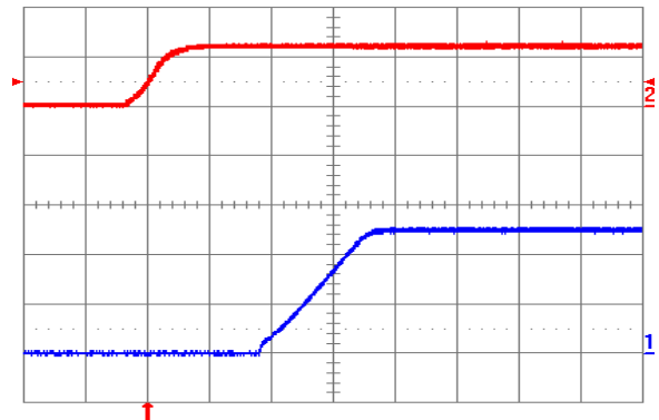
Fig. 2.5V.4: Turn-on transient for V_{out} = 2.5\text{ V} with application of V_{in} at full rated load current (resistive) and 100 \mu\text{F} external capacitance at V_{in} = 12\text{ V} . Top trace: V_{in} (10 V/div.); Bottom trace: output voltage (1 V/div.); Time scale: 2 ms/div.
