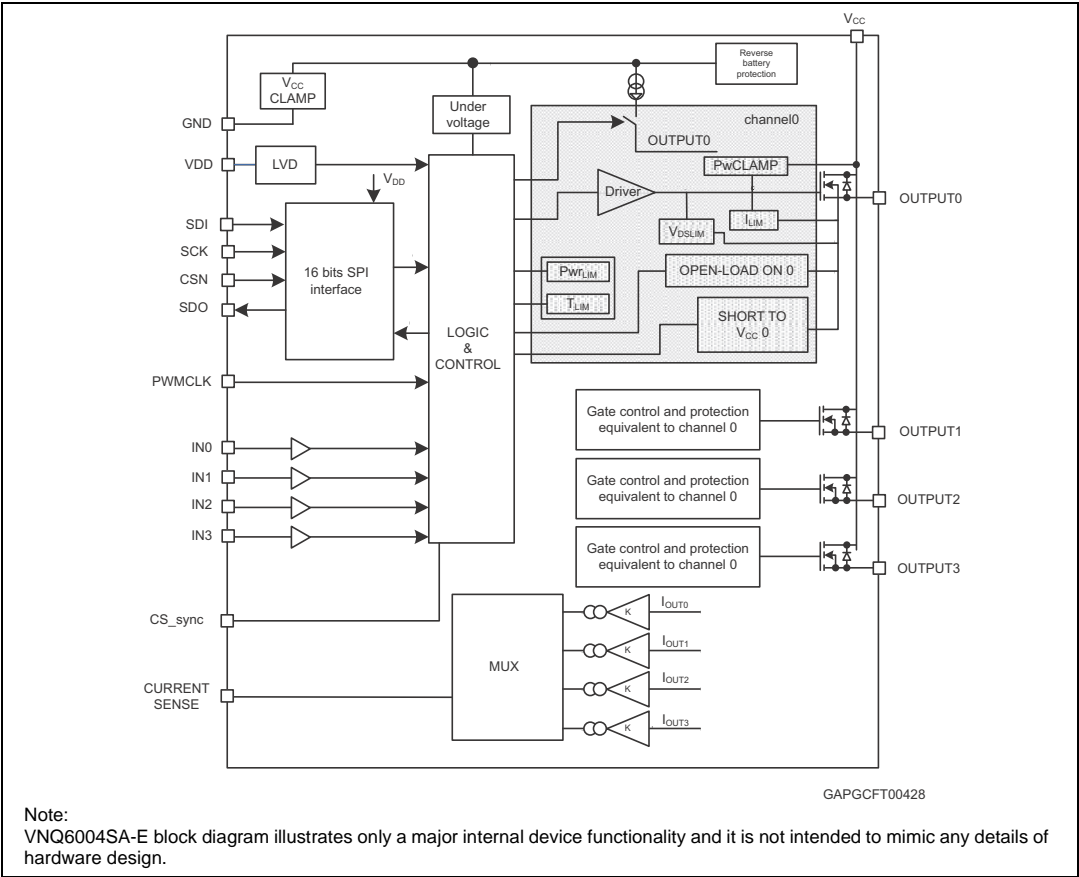
Figure 3. Block diagram
