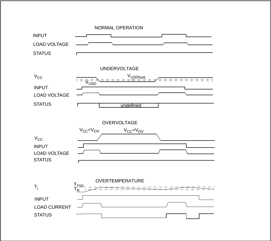
Figure 8. Waveforms
