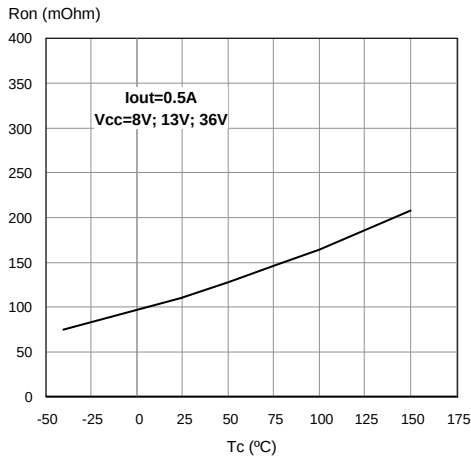
Figure 13. On-state resistance vs T_{case}
