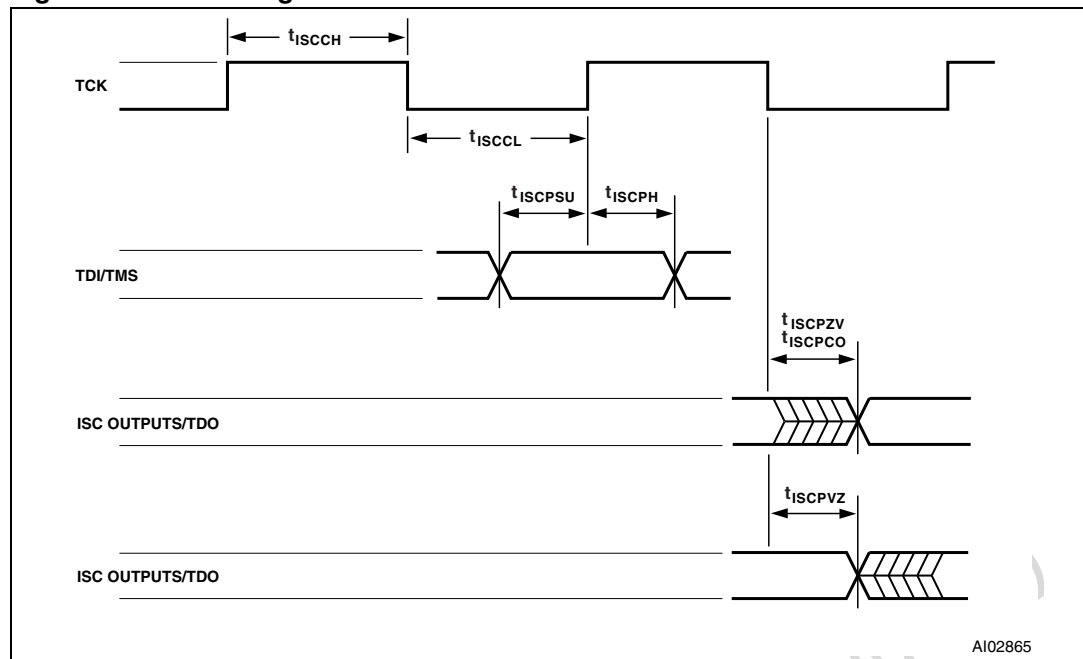
Figure 96. ISC timing
