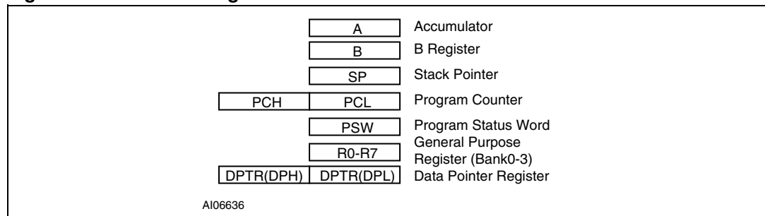
Figure 10. 8032 MCU registers
