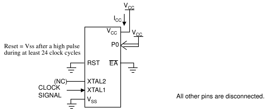
Figure 14-3. I_{CC} Test Condition, Idle Mode
