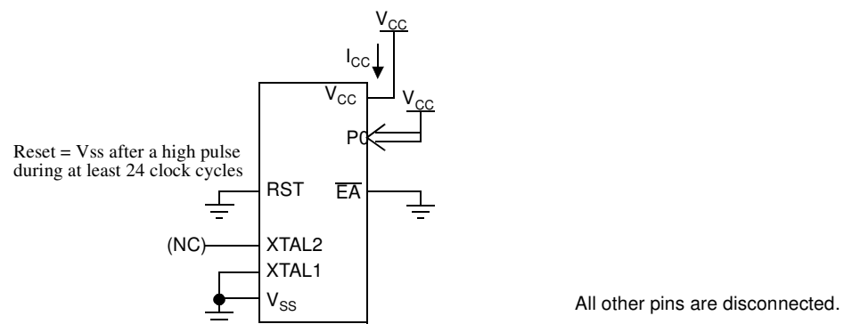
Figure 14-4. I_{CC} Test Condition, Power-Down Mode
