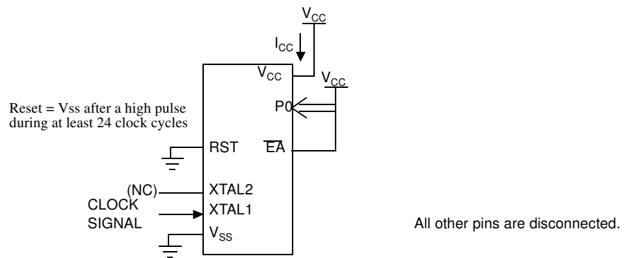
Figure 14-2. Operating I_{CC} Test Condition
