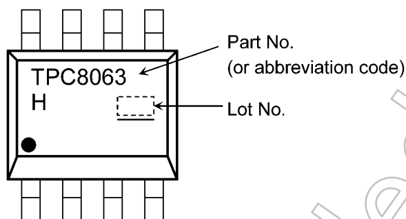
Fig. 7.1 Marking
