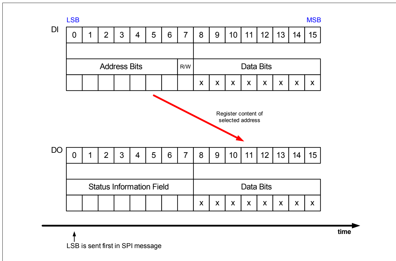
Figure 50 SPI Operation Mode
