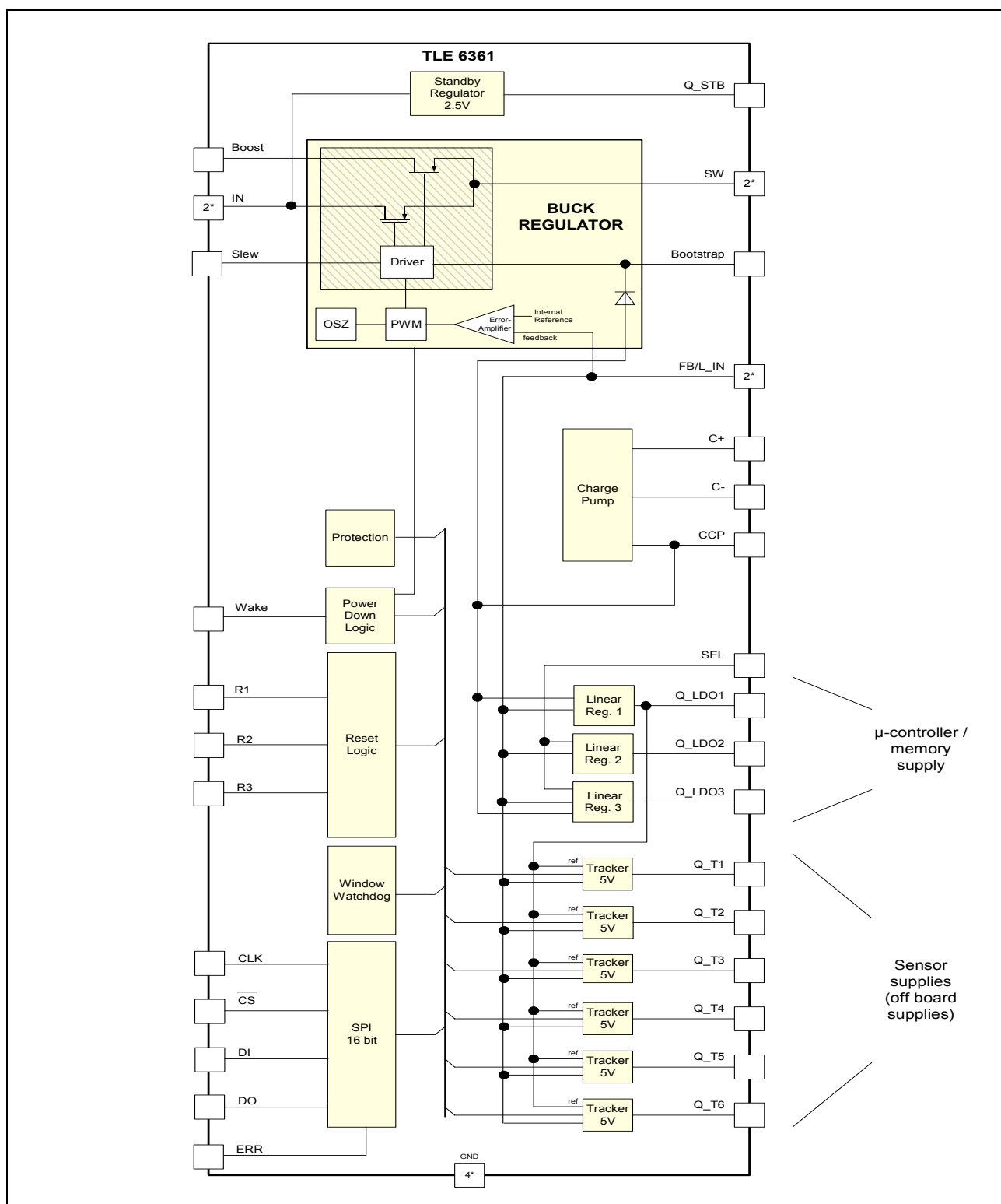
Figure 2 Block Diagram
