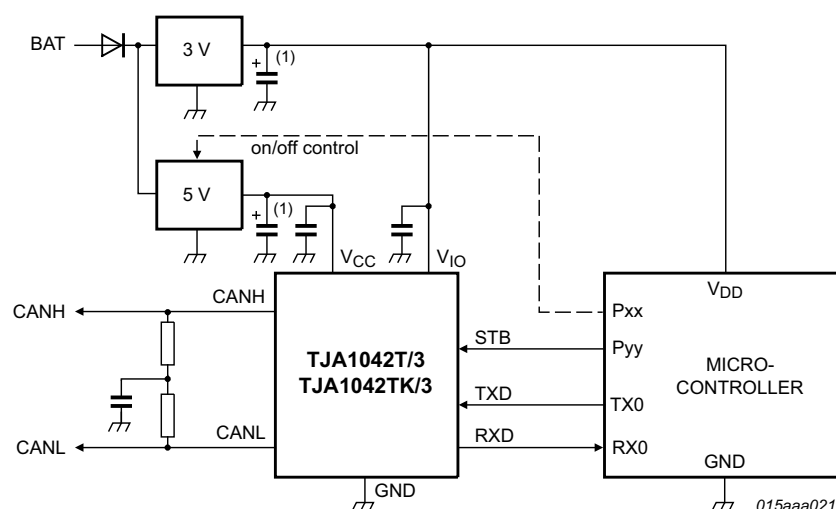
Fig 8. Typical application with TJA1042T/3 or TJA1042TK/3 and a 3 V microcontroller.
