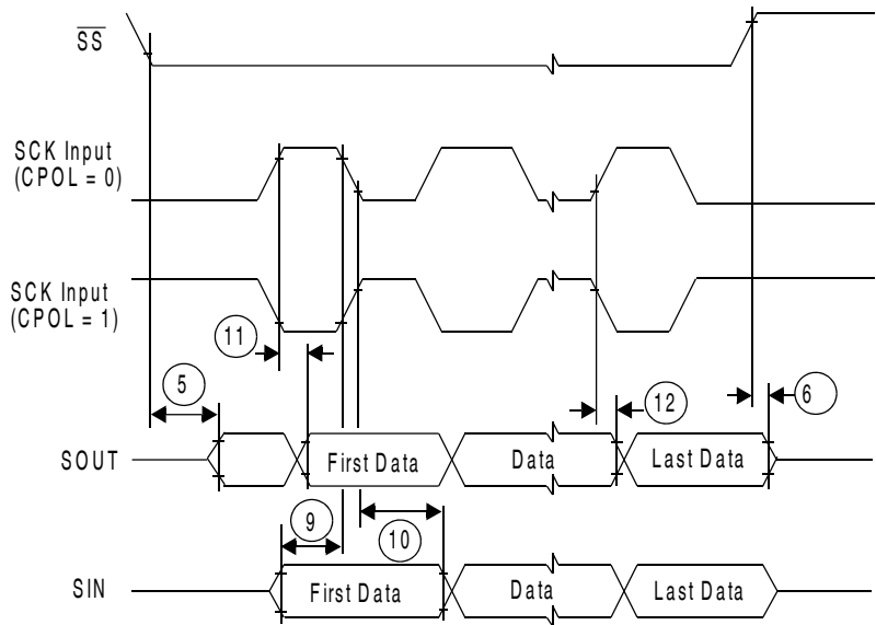
Figure 51. DSPI classic SPI timing slave, CPHA=1
