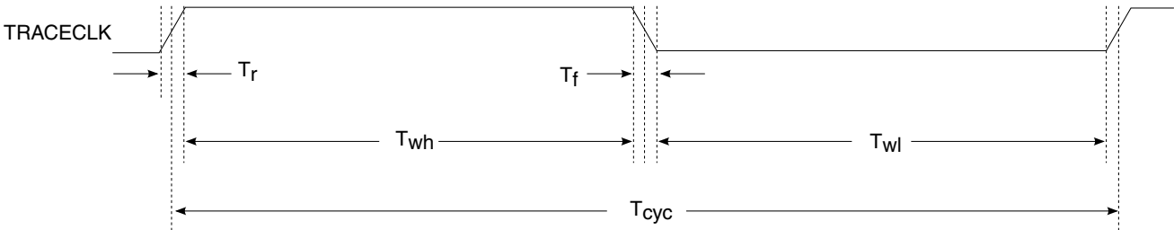
Figure 57. TRACE_CLKOUT specifications
