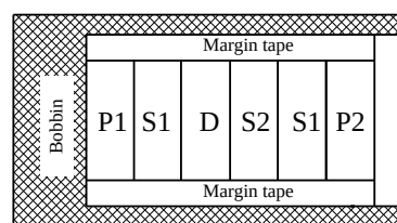
Winding structural example (b)
