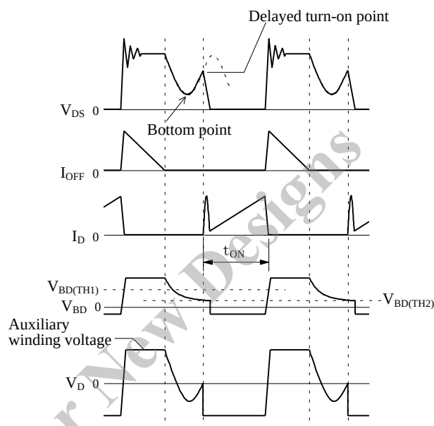
Figure 9-14 When the turn-on of a V_{DS} waveform occurs after a bottom point
