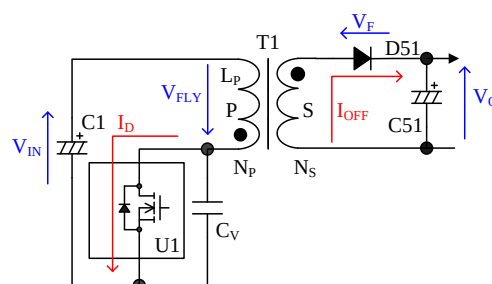
Figure 9-8 Basic flyback converter circuit
