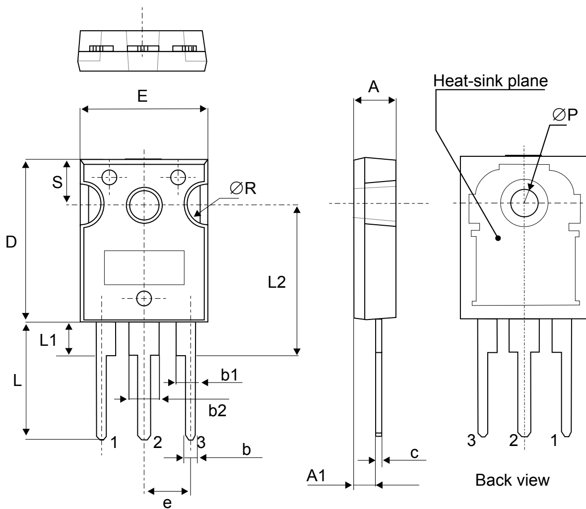
Figure 9. TO-247 package outline
