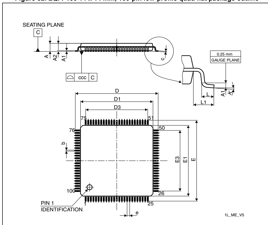
Figure 32. LQFP100 14 x 14 mm, 100-pin low-profile quad flat package outline
