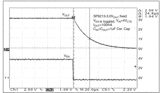
Turn off Time ( V_{IN} = 4V , I_{OUT} = 100mA )
