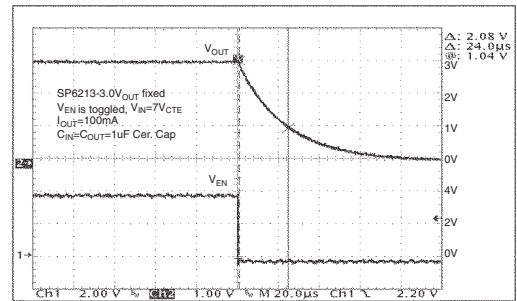
Turn off Time ( V_{IN} = 7V , I_{OUT} = 100mA )
