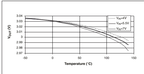
Output Voltage vs. Temperature ( I_{OUT} = 50mA )
