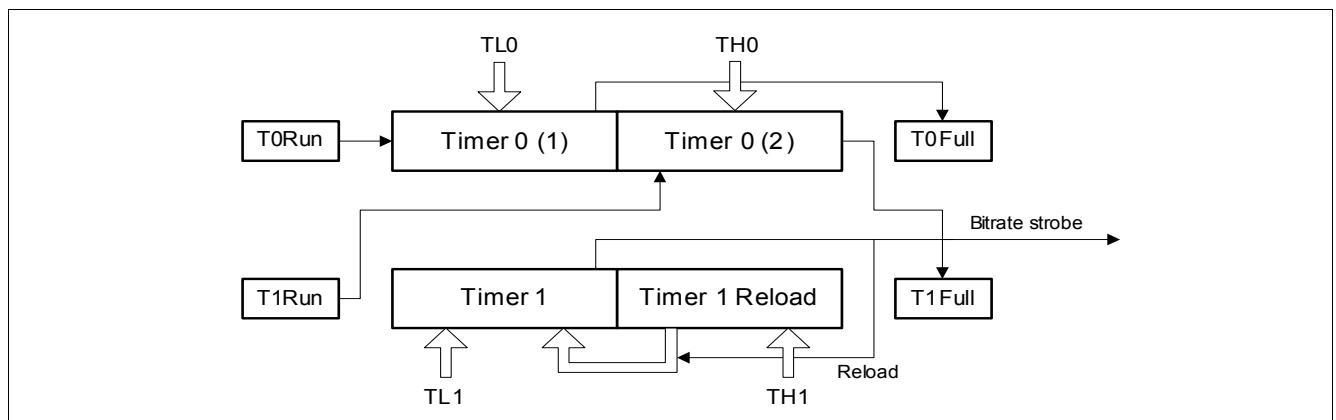
Figure 37 Timer Mode 3
