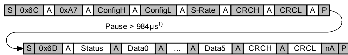
Figure 51 Measure Pressure
