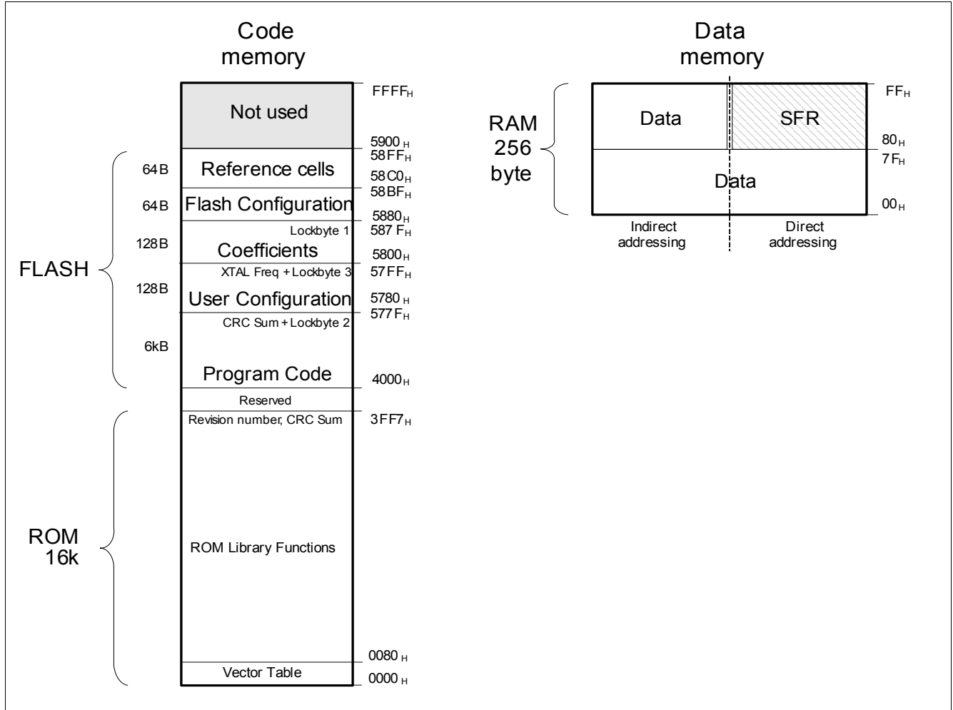
Figure 8 Memory Map
