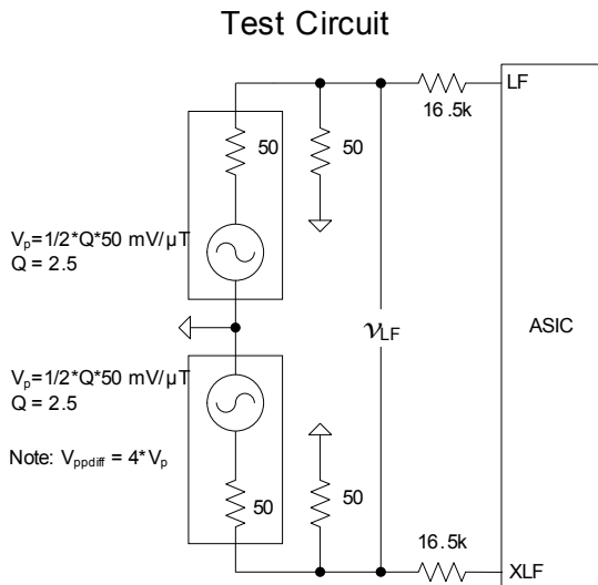
Figure 70 Test Circuit for large LF signal measurements
