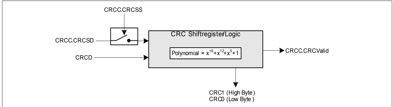
Figure 30 CRC (Cyclic Redundancy Check) Generator/Checker
