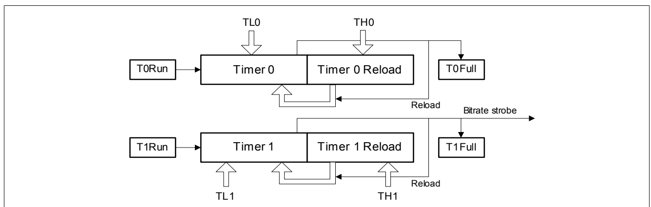
Figure 36 Timer Mode 2
