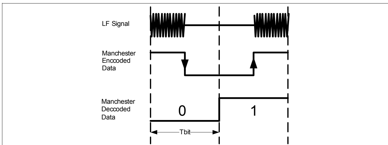
Figure 28 LF Decoder
