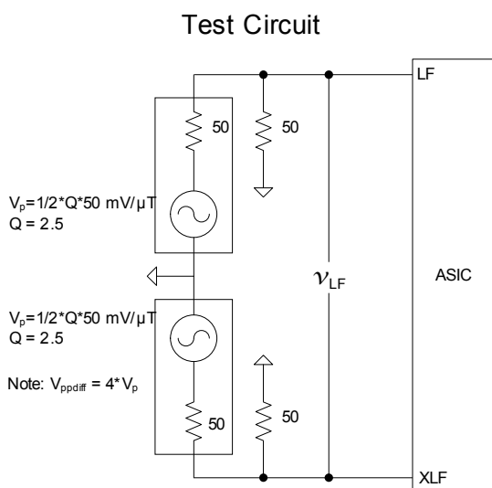
Figure 71 Test Circuit for small LF signal measurements
