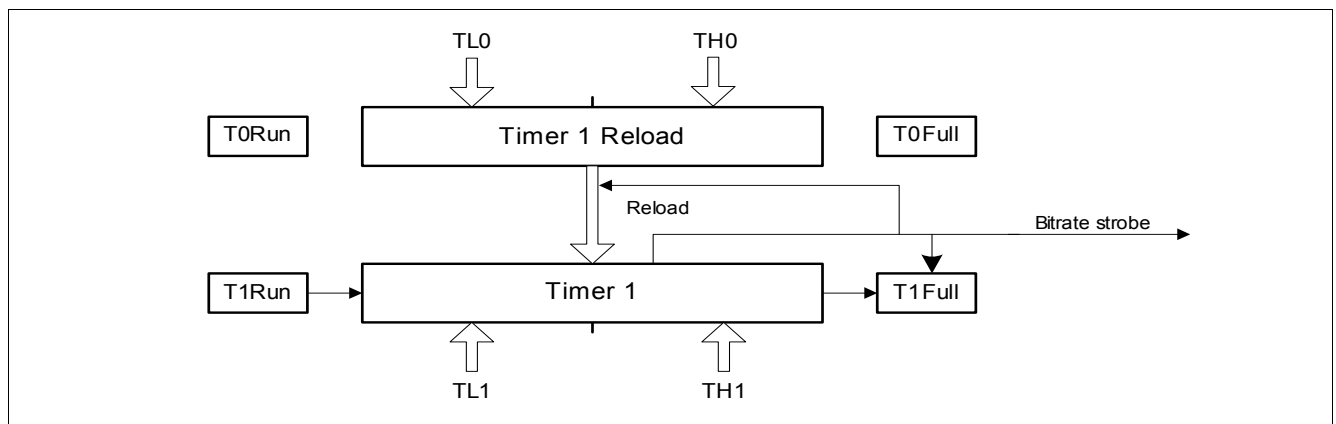
Figure 38 Timer mode 4
