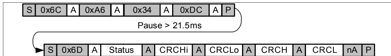
Figure 49 FLASH Check CRC
