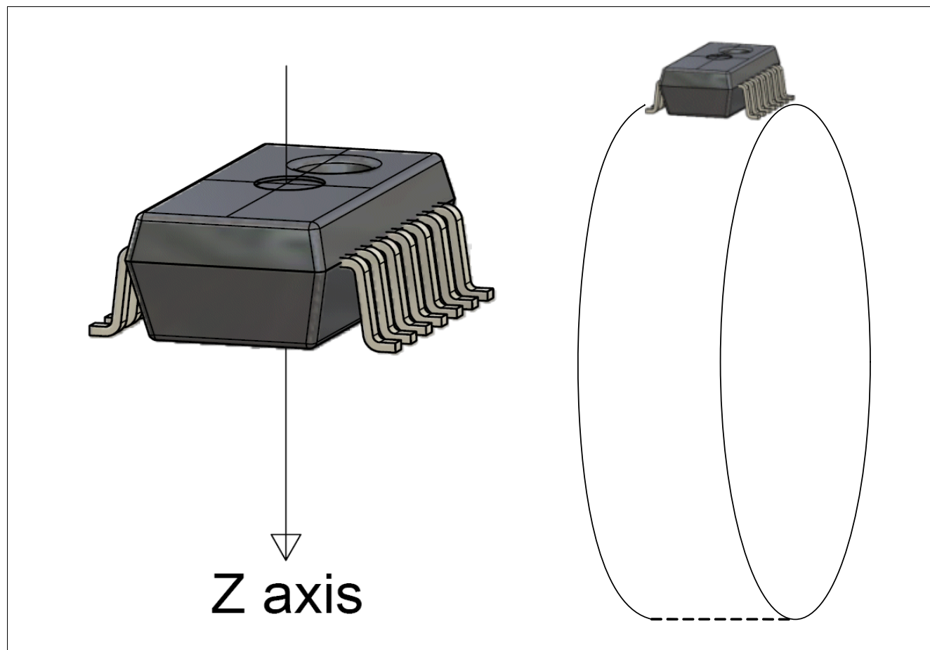
Figure 7 Device Orientation
