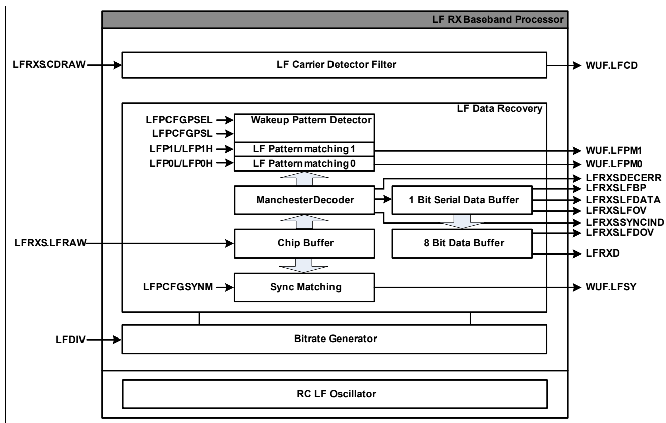
Figure 25 LF Receiver Baseband
