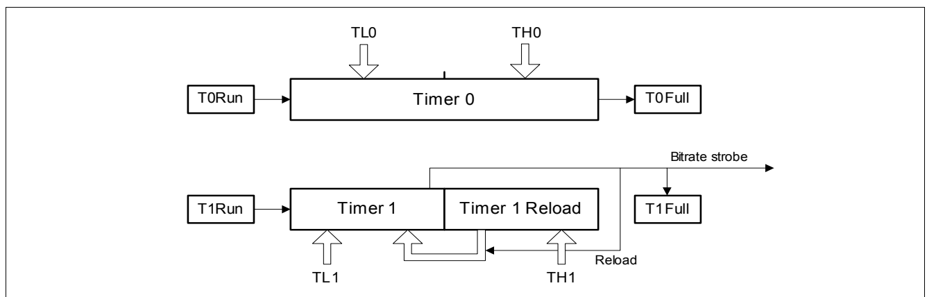
Figure 35 Timer Mode 1
