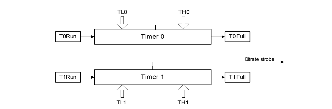
Figure 40 Timer Mode 6
