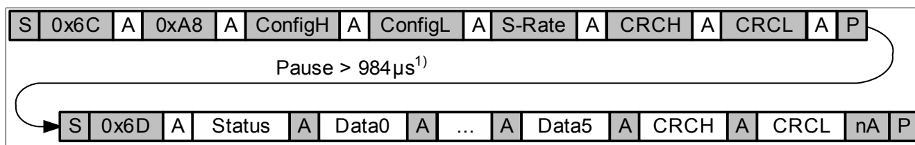
Figure 52 Measure Acceleration
