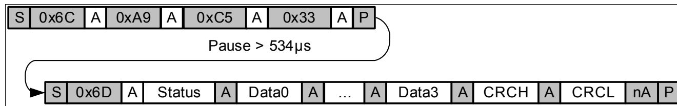
Figure 53 Measure Temperature
