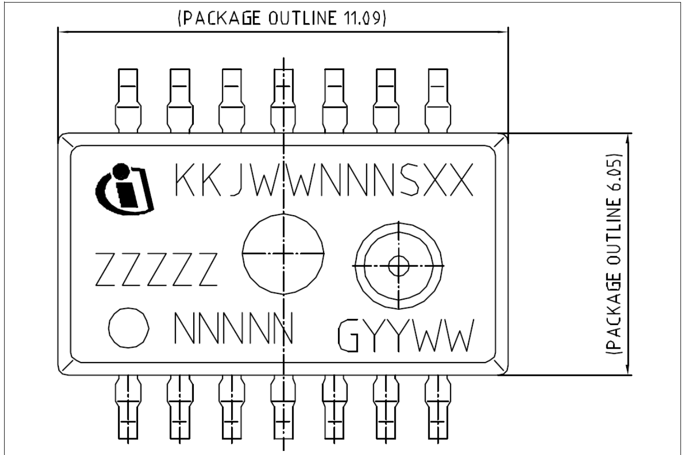
Figure 73 PG-DSOSP-14-6 marking
