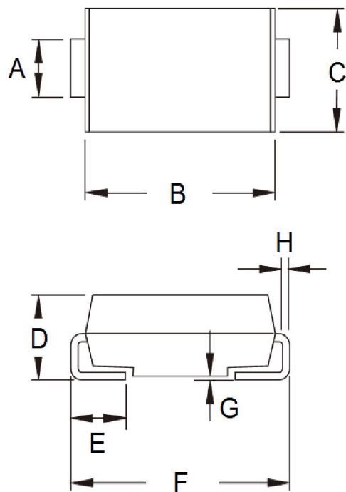
DO-214AA (SMB)
