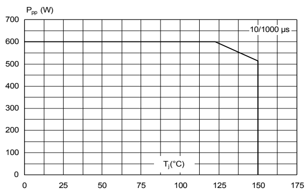
Figure 3. Maximum peak power dissipation versus initial junction temperature
