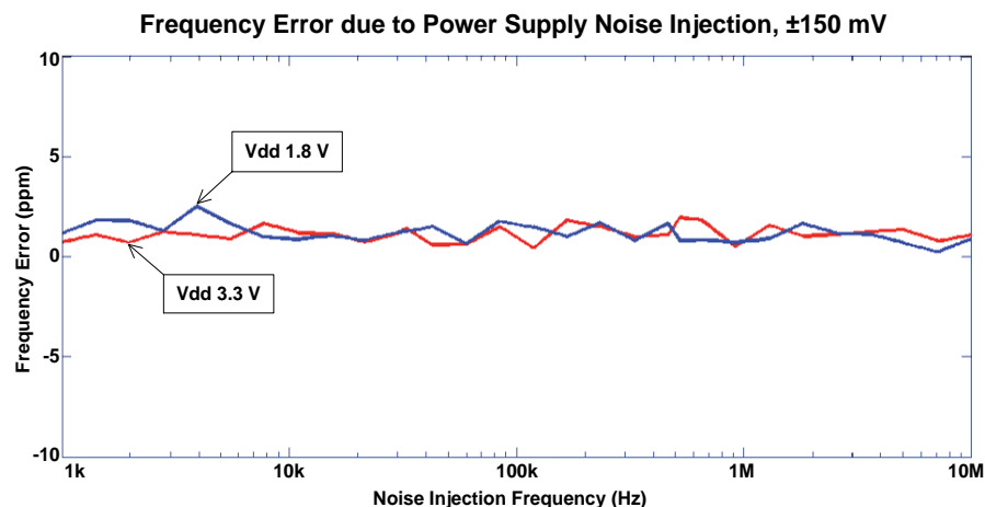
Figure 11. Power Supply Noise Rejection ( \pm 150 mV Noise)
