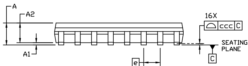
Figure 8.1. 16-Pin Narrow Body SOIC
