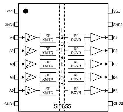
Figure 5.2. Si8655 Pinout
