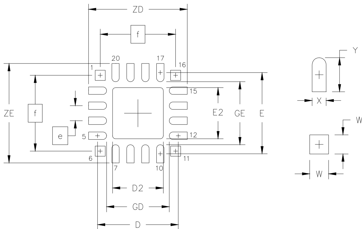
Figure 10. PCB Land Pattern
