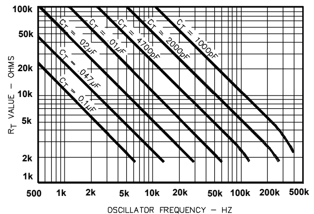
Figure 3 · Oscillator Frequency vs. R_T and C_T
