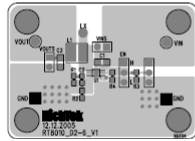
Figure 7. Top Layer
