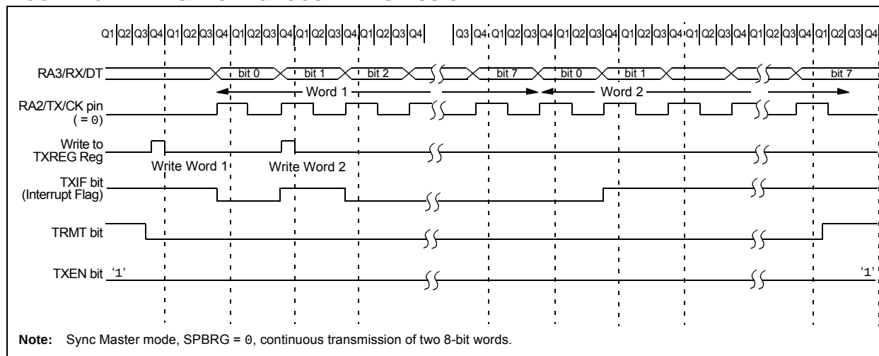
FIGURE 15-11: SYNCHRONOUS TRANSMISSION
