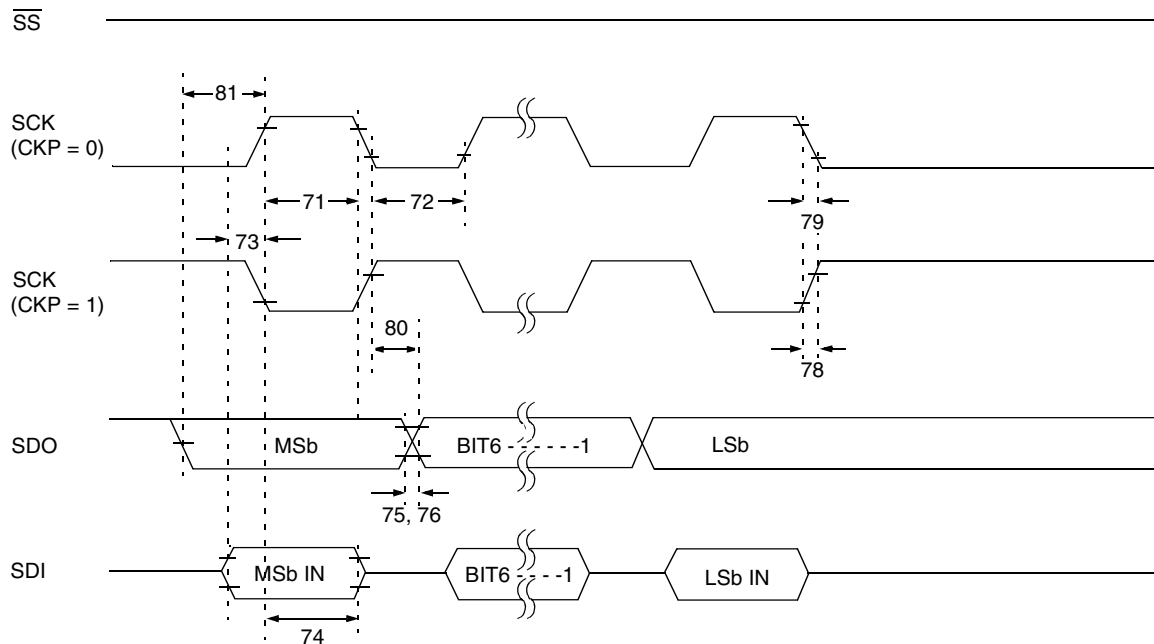
FIGURE 14-11: SPI MASTER MODE TIMING (CKE = 1, SMP = 1)
