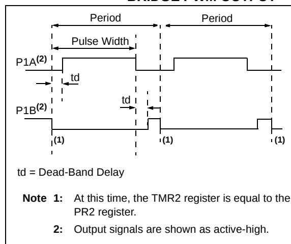
FIGURE 10-16: EXAMPLE OF HALF-BRIDGE PWM OUTPUT
