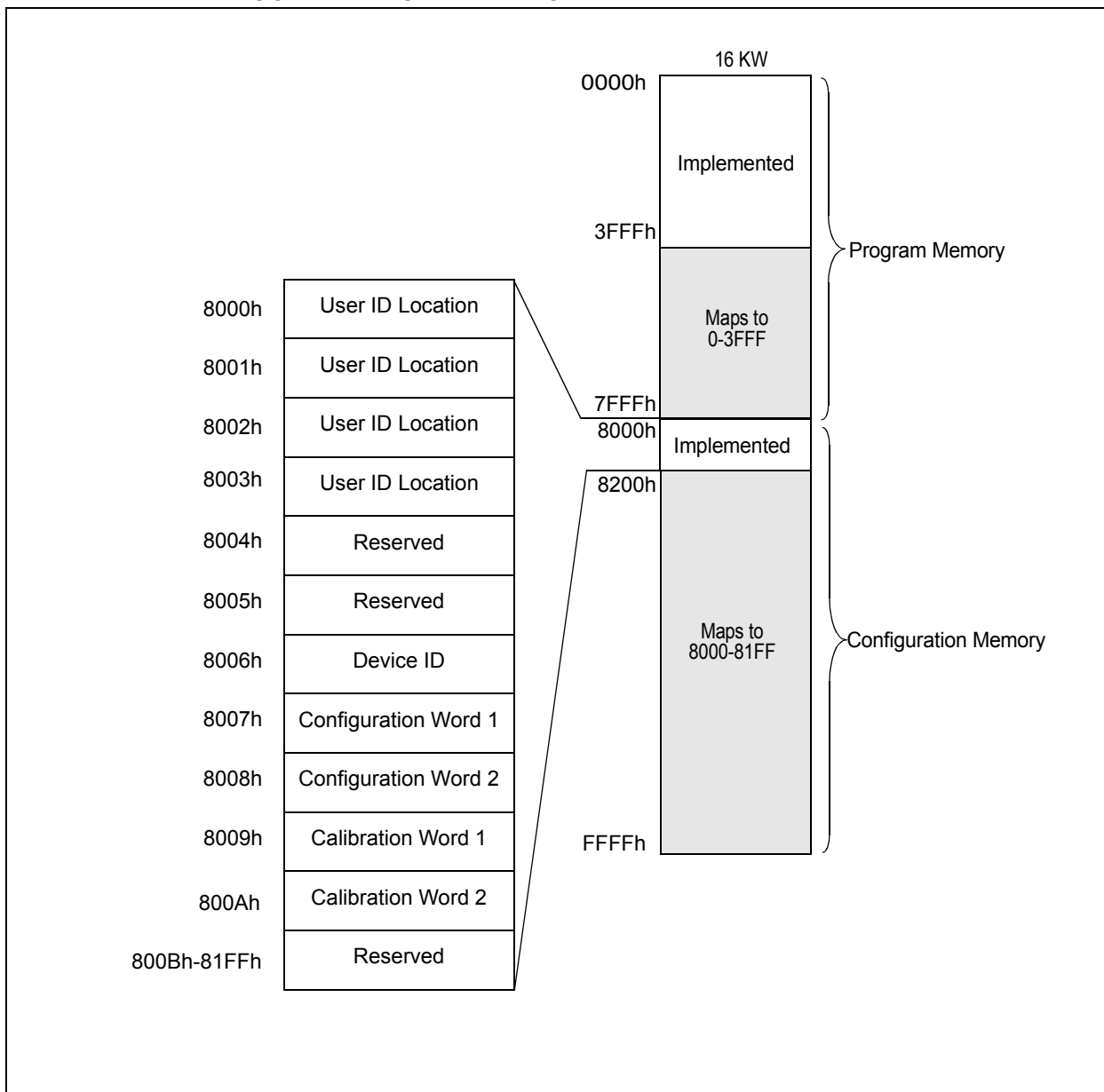
FIGURE 3-4: PIC16F1938/PIC16LF1938, PIC16F1939/PIC16LF1939, PIC16F1947/PIC16LF1947 PROGRAM MEMORY MAPPING
