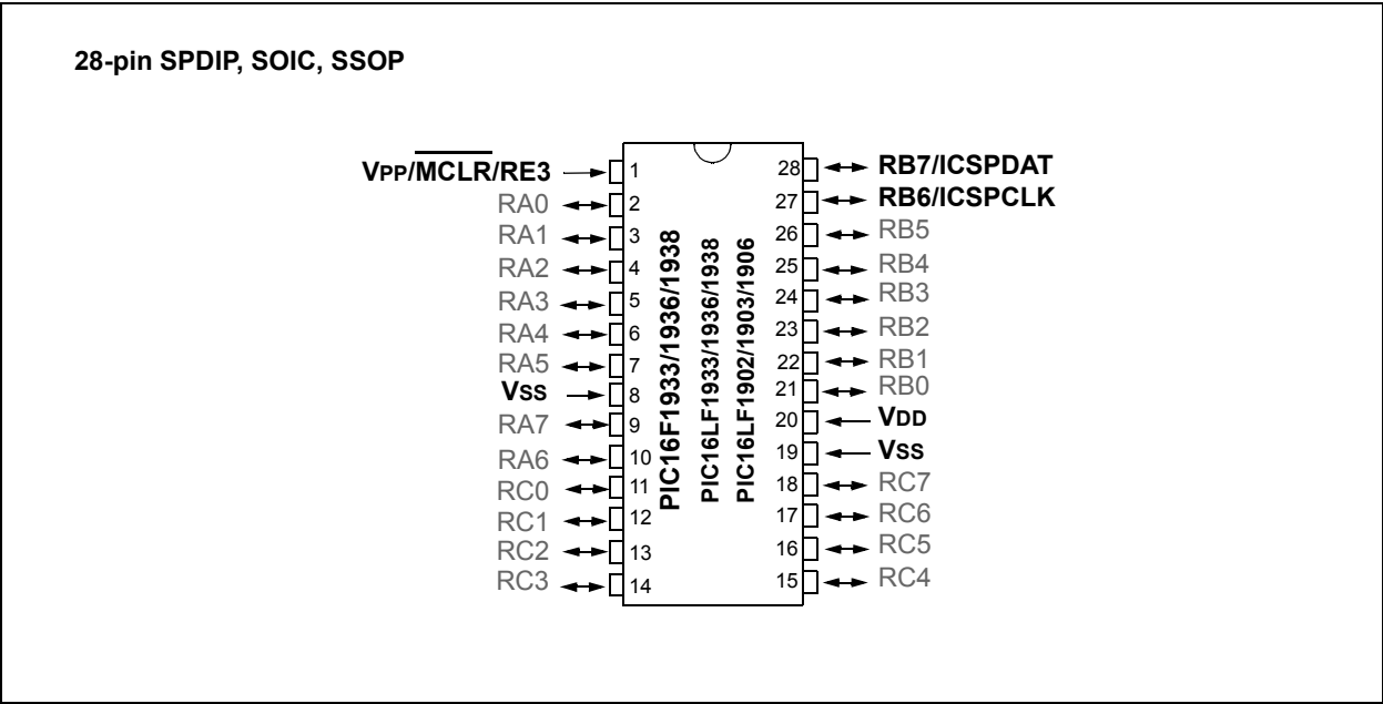
FIGURE 2-1: 28-PIN PDIP/SOIC/SSOP DIAGRAM FOR PIC16F1933/1936/1938, PIC16LF1933/1936/1938 AND PIC16LF1902/1903/1906
