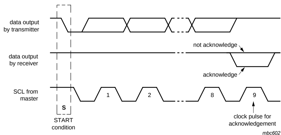
Fig 17. Acknowledgement on the I 2 C-bus
