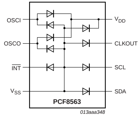
Fig 23. Device diode protection diagram
