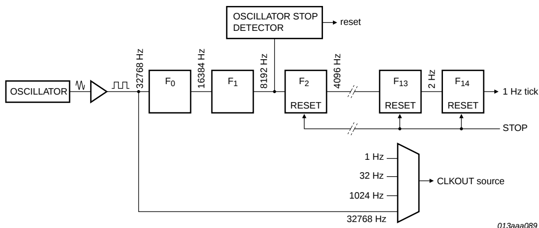
Fig 11. STOP bit functional diagram
