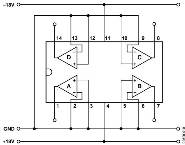
Figure 19. Burn-In Circuit
