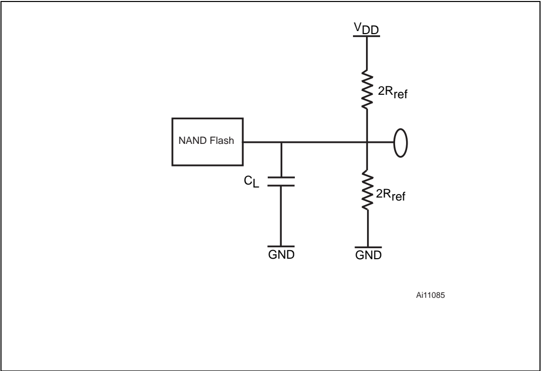
Figure 20. Equivalent testing circuit for AC characteristics measurement
