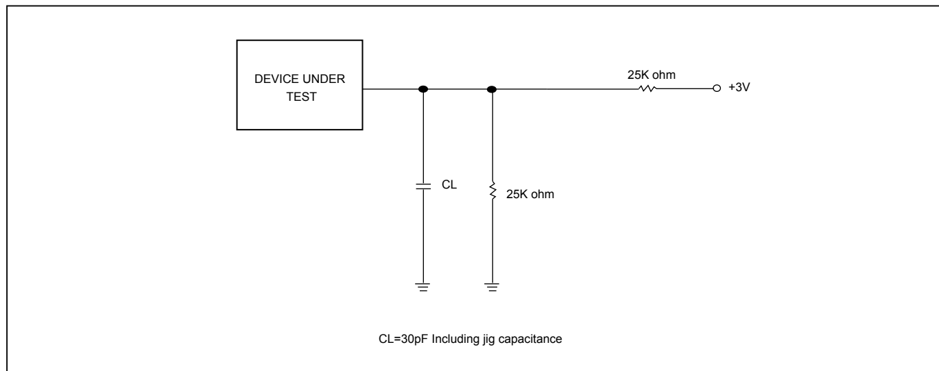
Figure 95. OUTPUT LOADING
