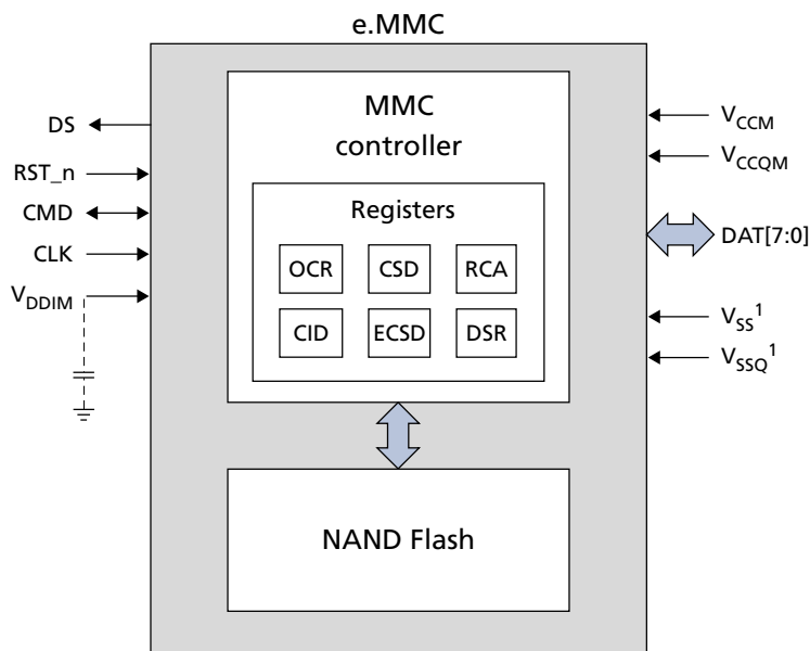
Figure 7: e.MMC Functional Block Diagram
