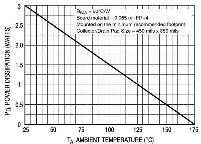
Figure 15. D²PAK Power Derating Curve
