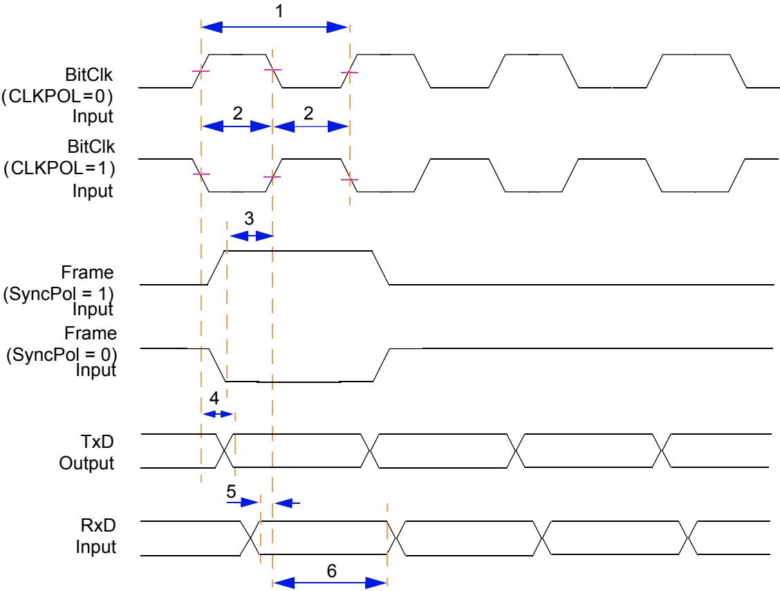
Figure 39. Timing Diagram — 8,16, 24, and 32-bit CODEC / I²S Slave Mode
