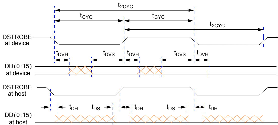
Figure 18. Timing Diagram—Sustained Ultra DMA Data In Burst
