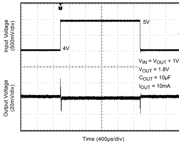
Line Transient
