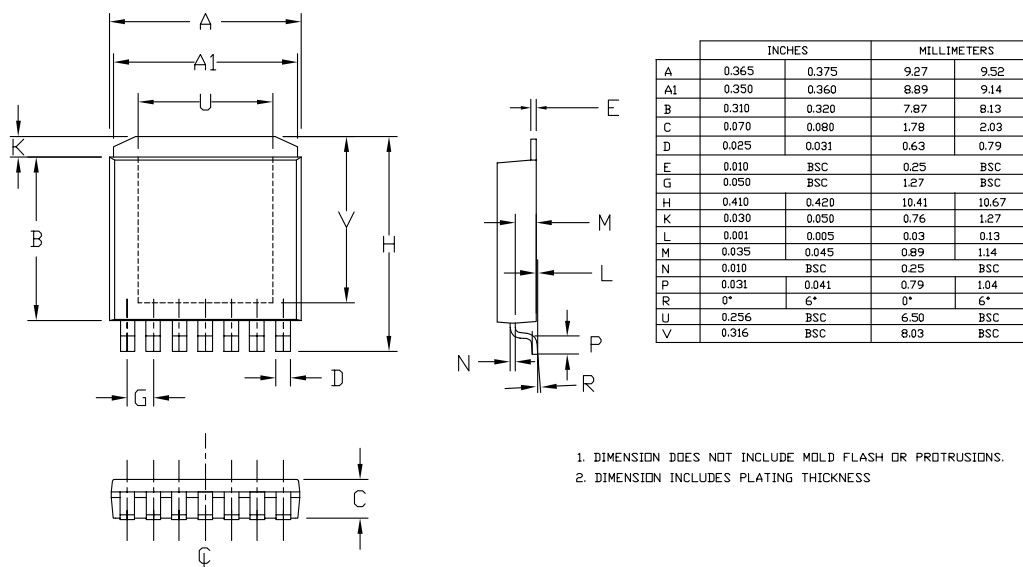
7-Pin S-PAK (R)
