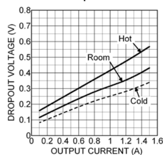
MIC29152 Dropout Voltage vs. Output Current
