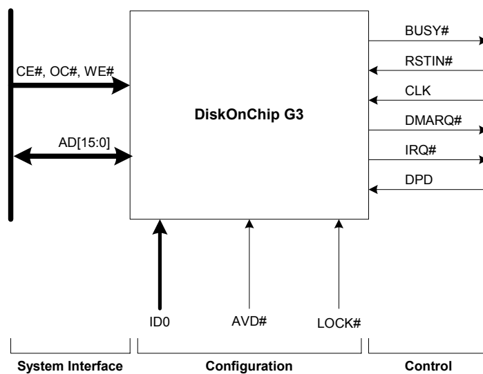
Figure 10: Multiplexed Interface Simplified I/O Diagram (DiskOnChip G3 128MB/1Gb 9x12 FBGA Package)
