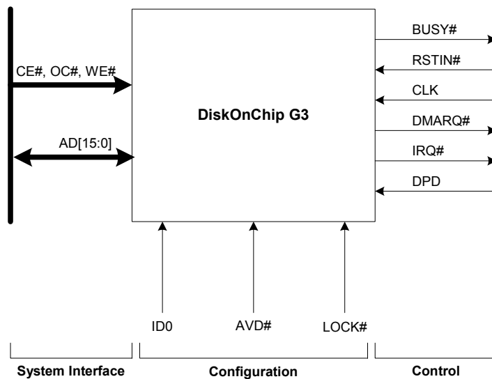
Figure 8: Multiplexed Interface Simplified I/O Diagram (DiskOnChip G3 64MB/512Mb 7x10 FBGA Package)
