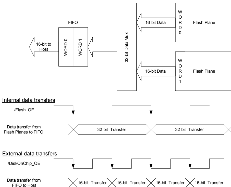
Figure 15: MultiBurst Operation
