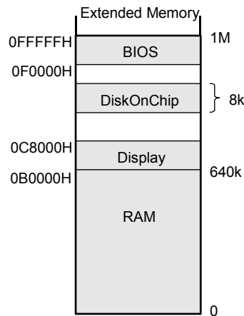
Figure 20: DiskOnChip G3 Memory Window in PC Memory Map
