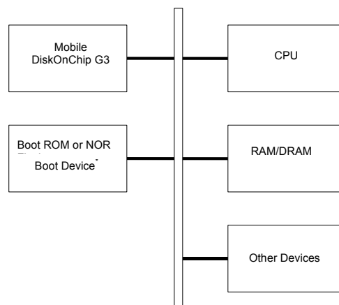
Figure 21: Typical System Architecture Using DiskOnChip G3
