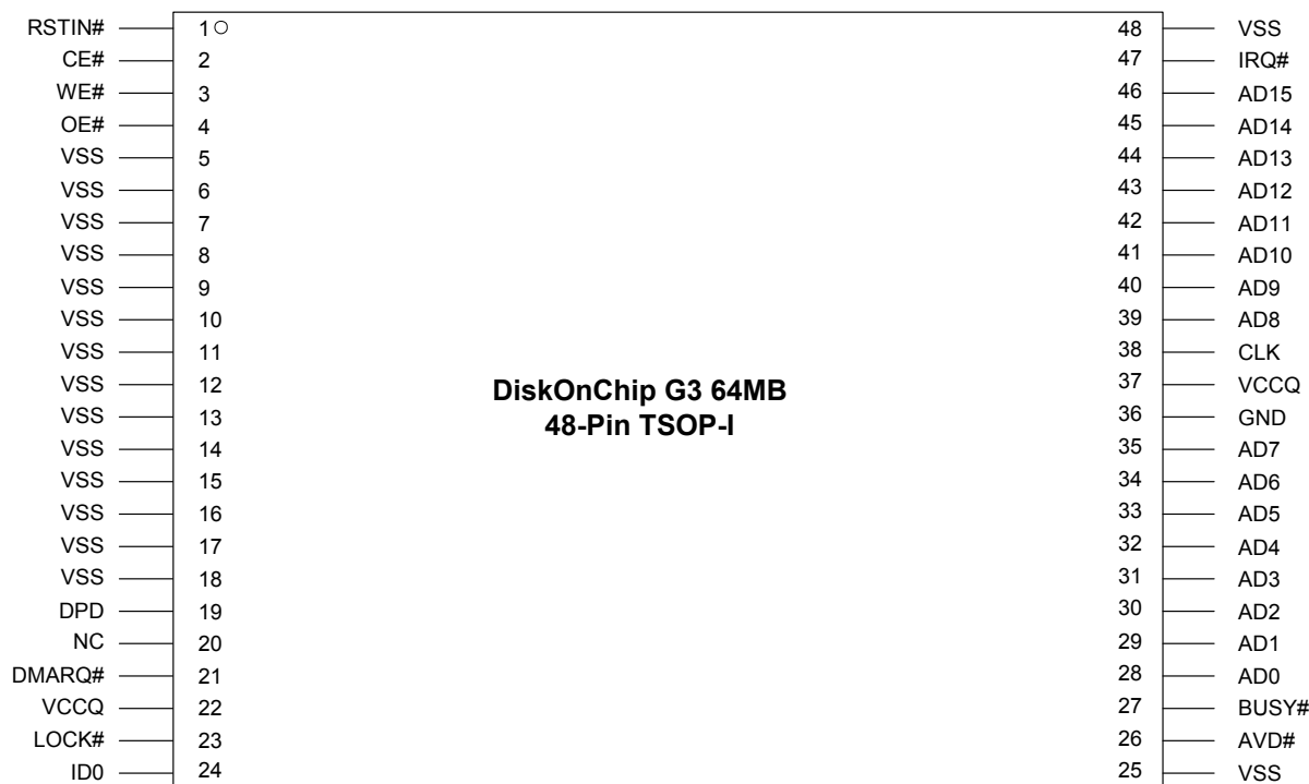
Figure 6: Pinout for Multiplexed Interface (DiskOnChip 64MB/512Mb TSOP-I Package)
