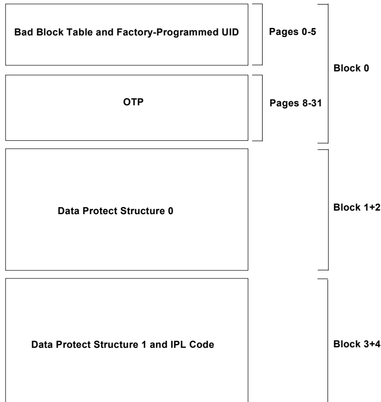
Figure 16: Low Level Structure of DiskOnChip G3
