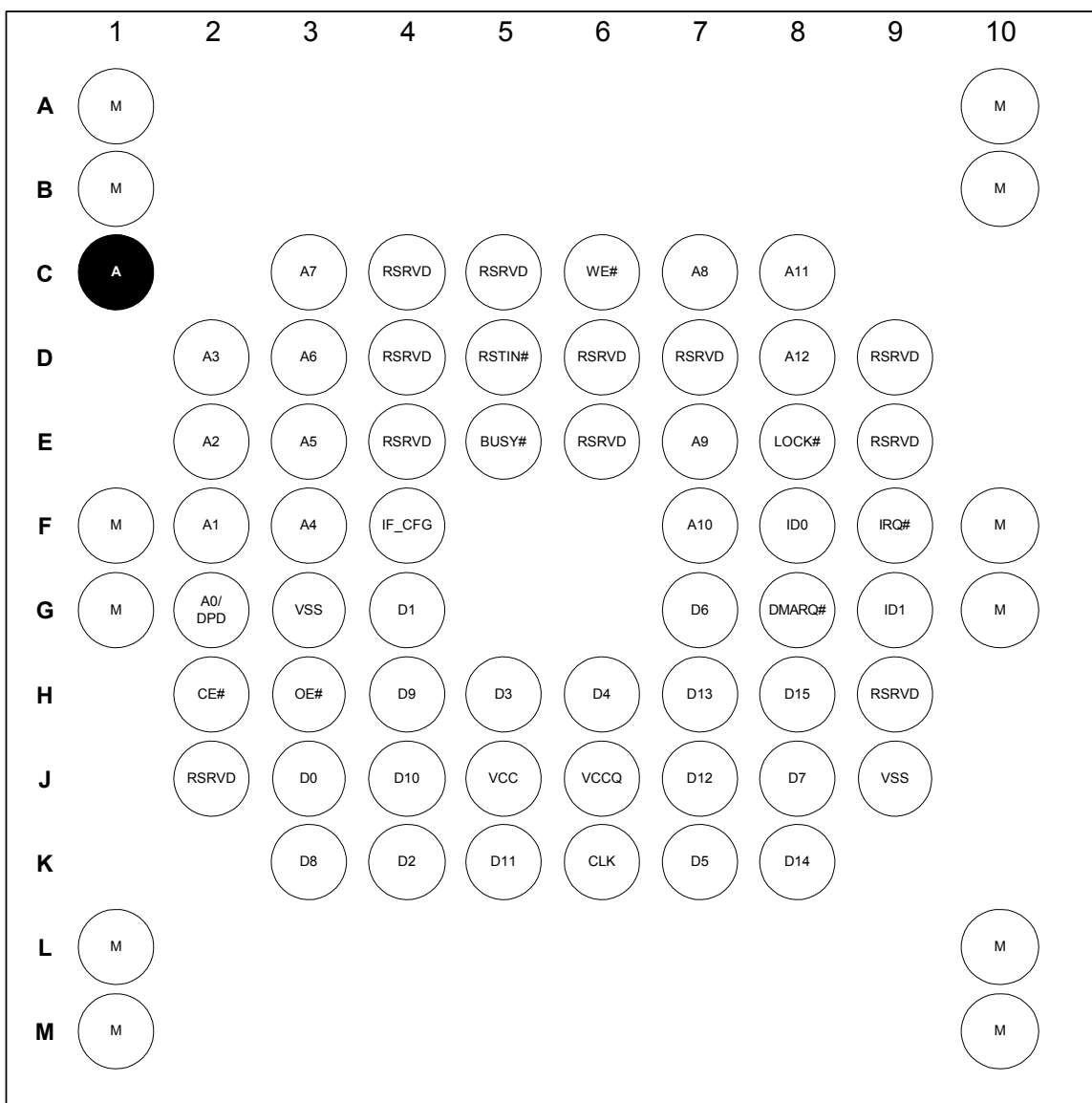
Figure 4 Ballout for Standard Interface (DiskOnChip G3 128MB/1Gb 9x12 FBGA Package)
