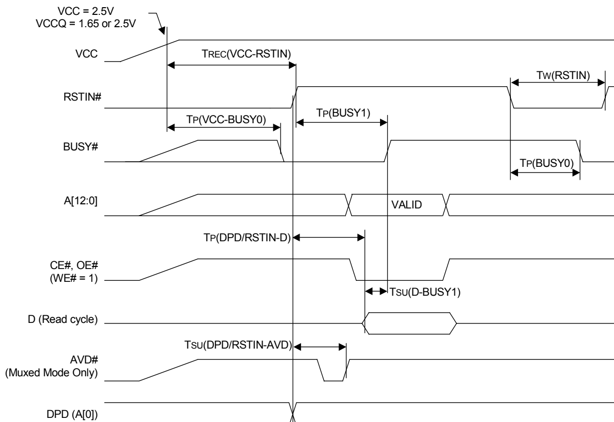
Figure 33: Reset Timing
