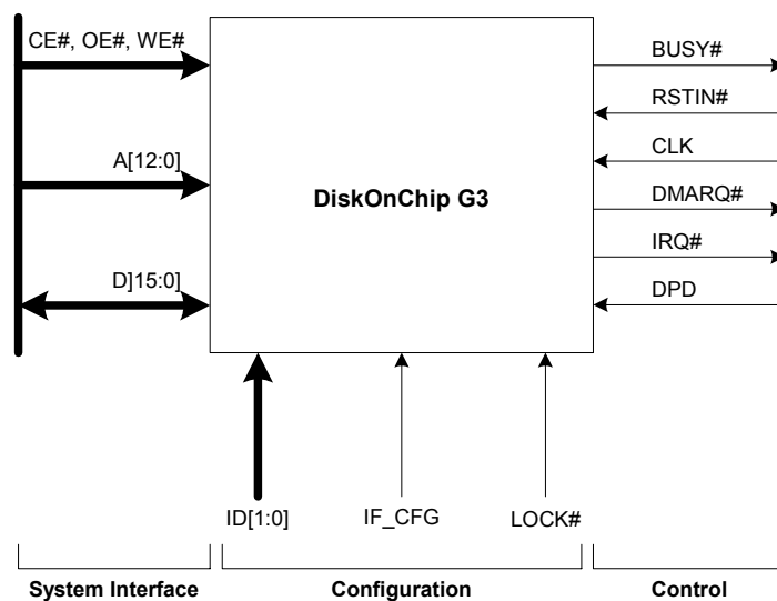
Figure 3: Standard Interface Simplified I/O Diagram (DiskOnChip G3 64MB/512Mb)
