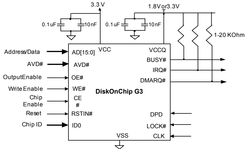
Figure 23: Multiplexed System Interface
