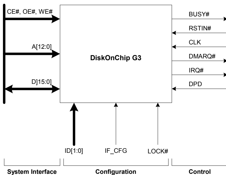
Figure 5: Standard Interface Simplified I/O Diagram (DiskOnChip G3 128MB/1Gb)
