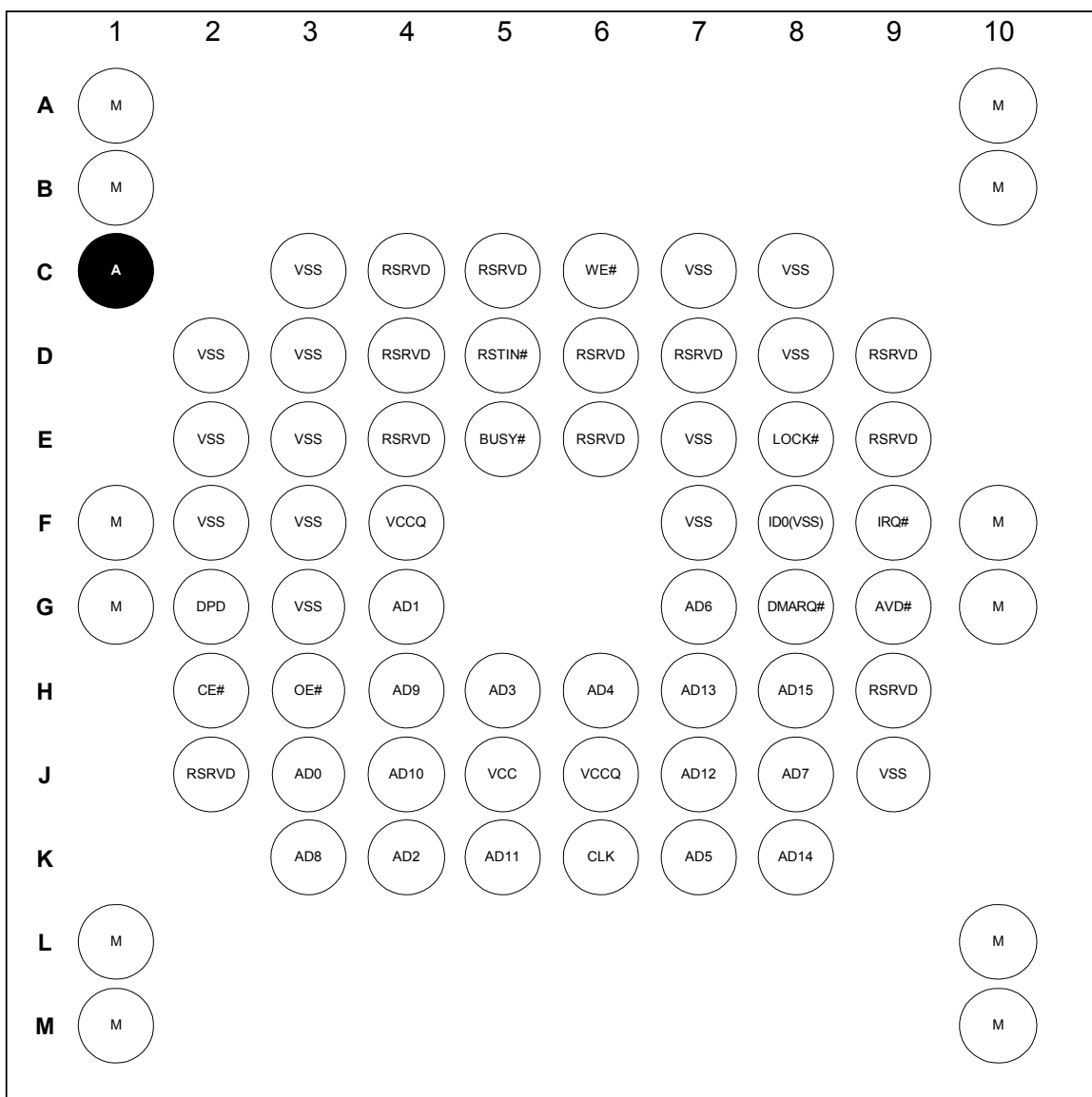
Figure 9: Ballout for Multiplexed Interface (DiskOnChip G3 128MB/1Gb 9x12 FBGA Package)
