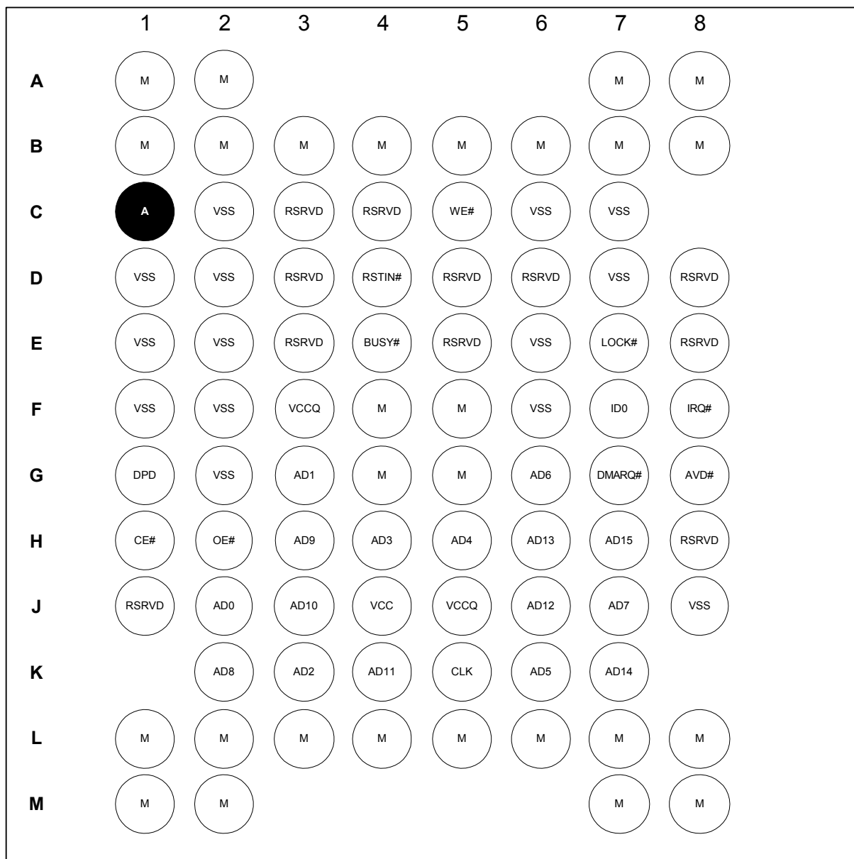
Figure 7 Ballout for Multiplexed Interface (DiskOnChip 64MB/512Mb 7x10 FBGA Package)
