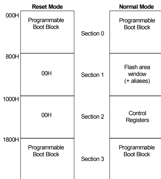
Figure 19: DiskOnChip G3 Memory Map
