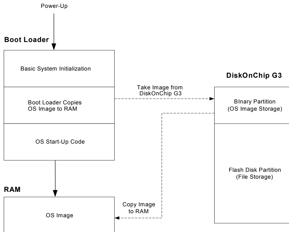
Figure 25: System Boot Flow with DiskOnChip G3
