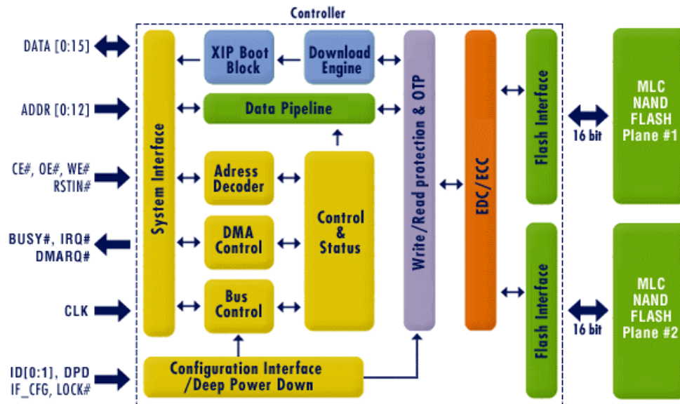
Figure 11: DiskOnChip G3 Simplified Block Diagram, Standard Interface
