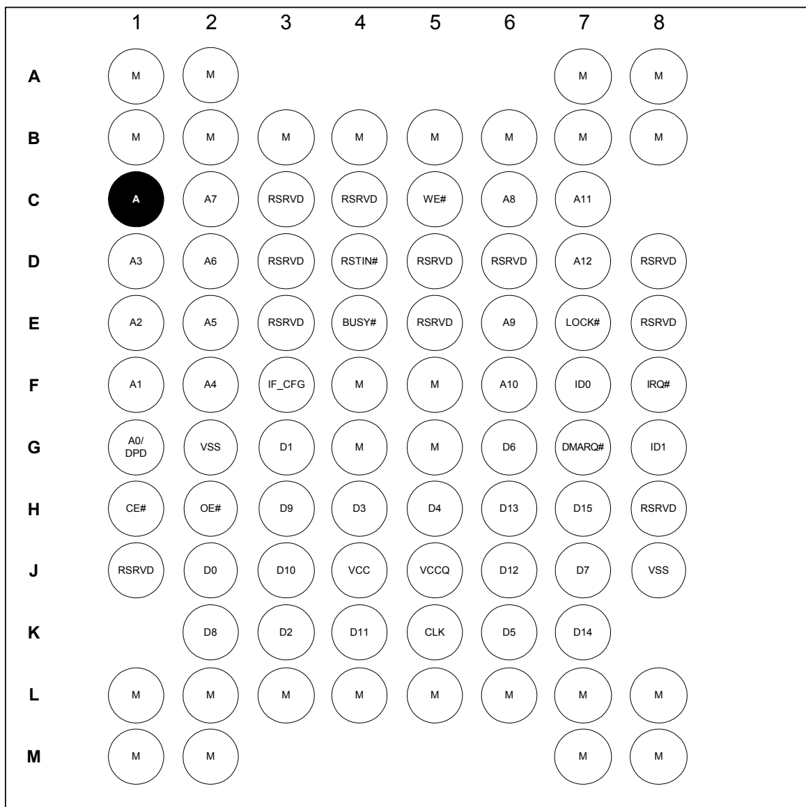
Figure 2: 7x10 FBGA Ballout for Standard Interface (DiskOnChip G3 64MB/512Mb)
