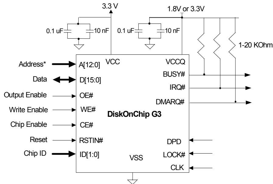
Figure 22: Standard System Interface
